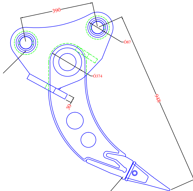
CAT 225 TOOTH ASSEMBLY
